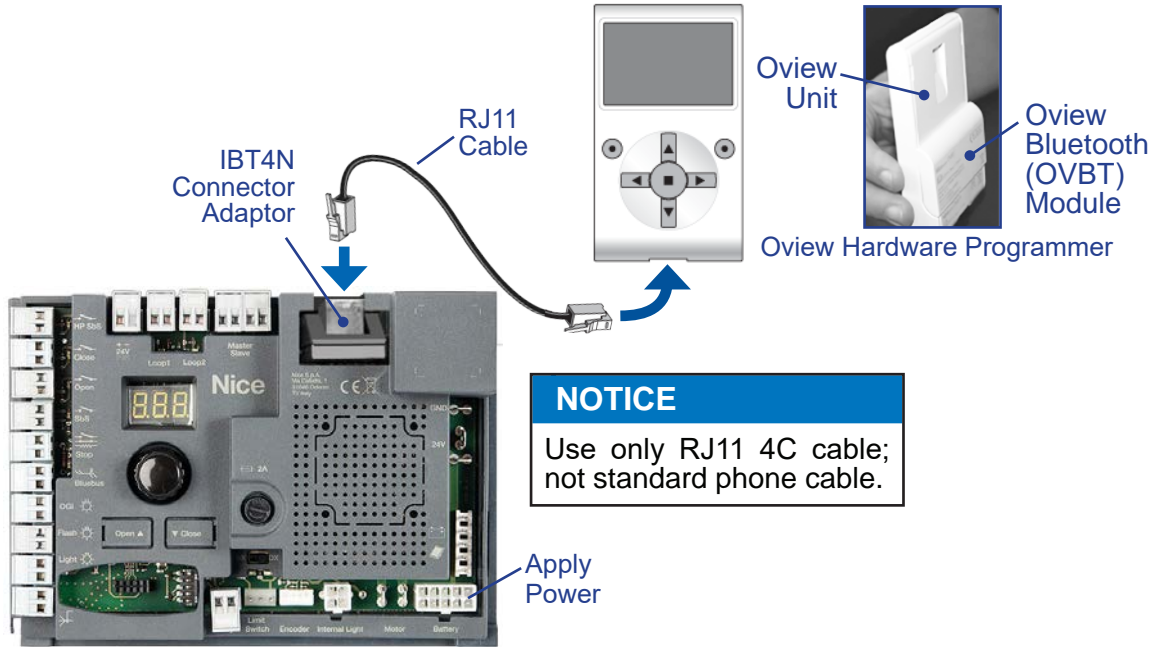
Fig-1: BCU1 Controller Update Setup
