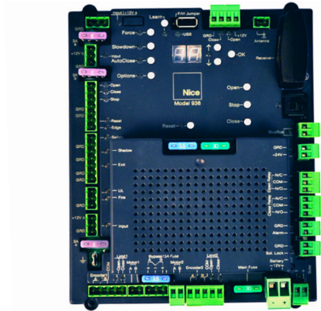
936US Control Board
